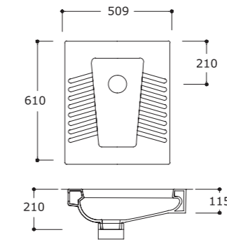
TP02HLT00 ÇEVRE YIKAMALI HELA TAŞI TP02HLT00 SQUATTING PAN BOX RIM
