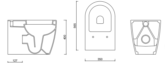
UN03DTK00 UNO DUVARA DAYALI TEK KLOZET
