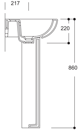
K005LVB01 COMPACT WASHBASIN (50x60)
