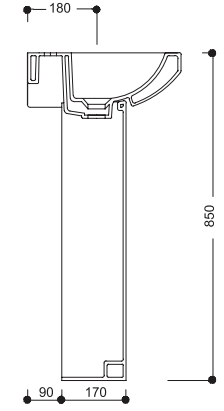
NE12LVB01 NERO WASHBASIN (40x55)
